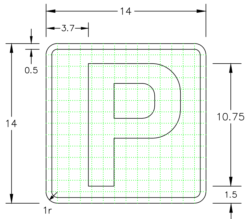
Tile used on Informatory & Directional signs
